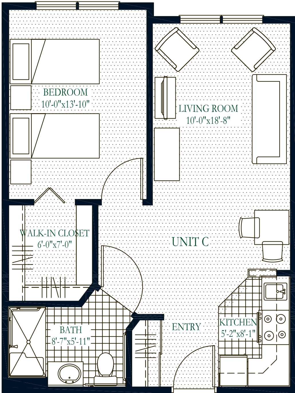
UNIT C FLOOR PLAN 1 BEDROOM / 1 BATH 577 SF
