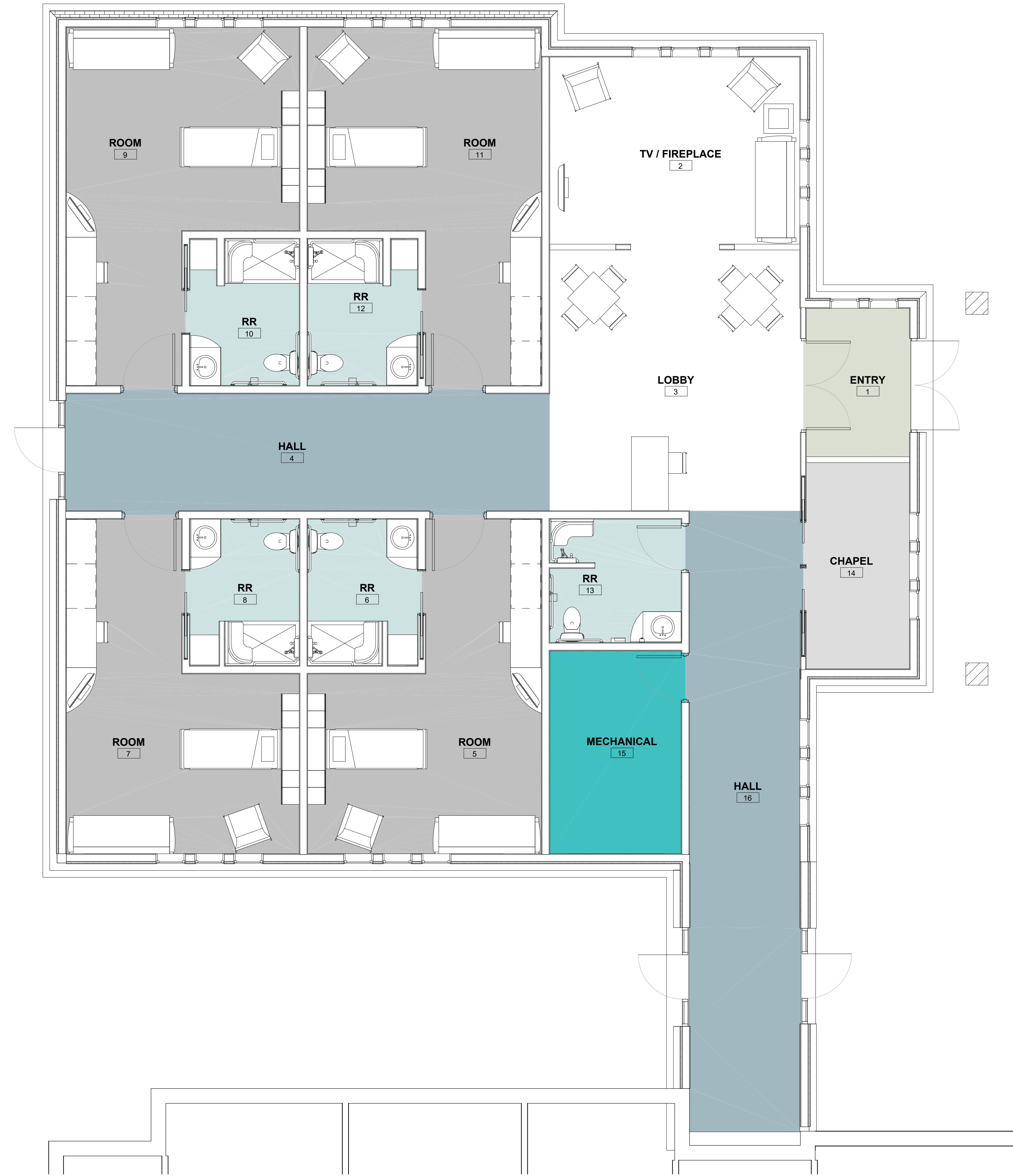
1 MAIN LEVEL FLOOR PLAN A100 1/4" = 1'-0"
